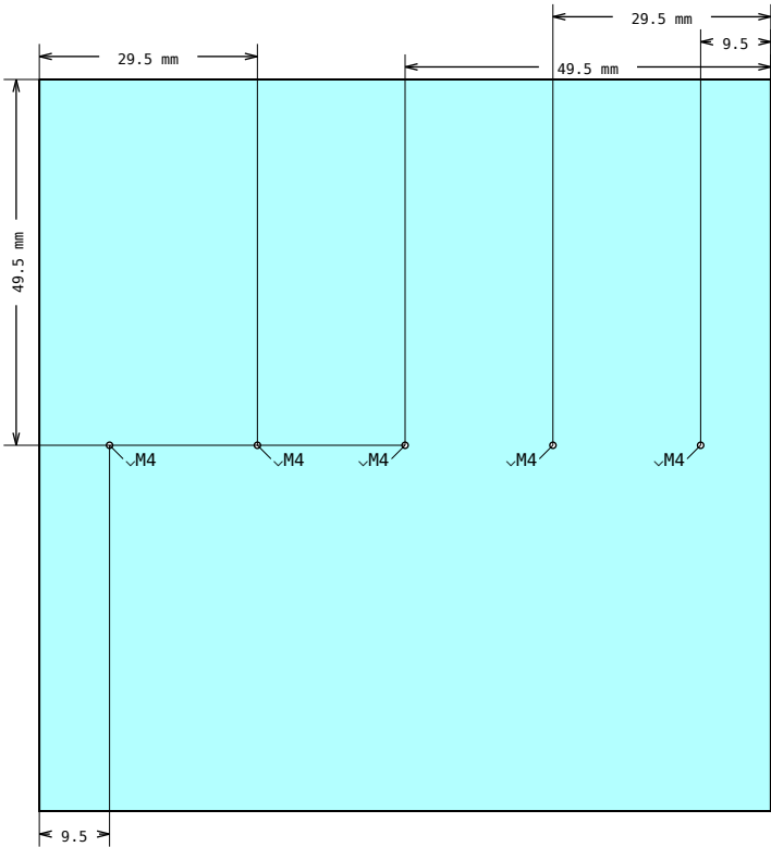
DRAWING 3, Pos 6 Hole placement
